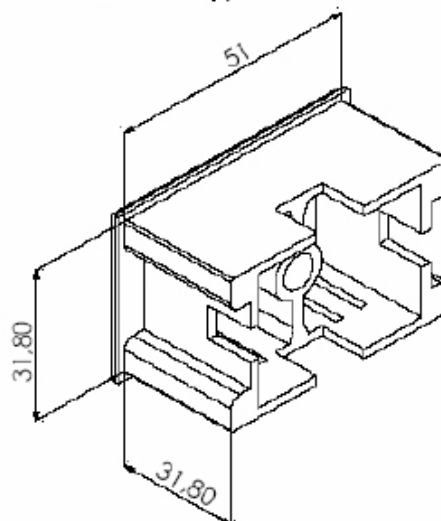
NYL 28.025 TAMPA 1 1/4" x 2"
